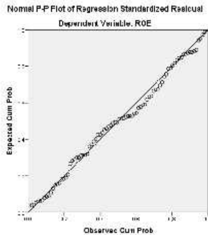
Gambar 2 : Probability Plot
